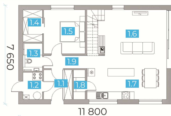
Parter 74,02 m 2
